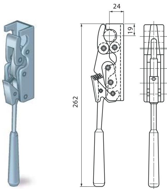
15001540 Chiusura universal kg 1,210
