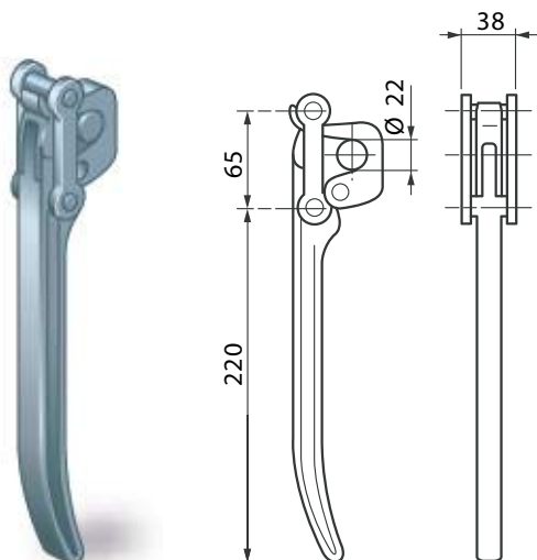
15001520 Leva marotta Ø 22 kg 1,370
