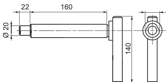
25021520 Spina Ø 31 a 2 fresature 1,380 kg
